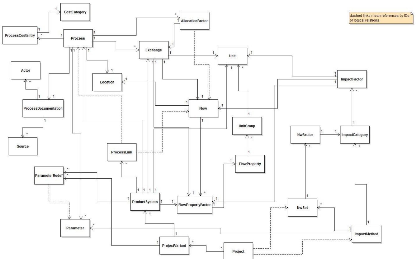
Figure 157: Classes and dependencies of core model
