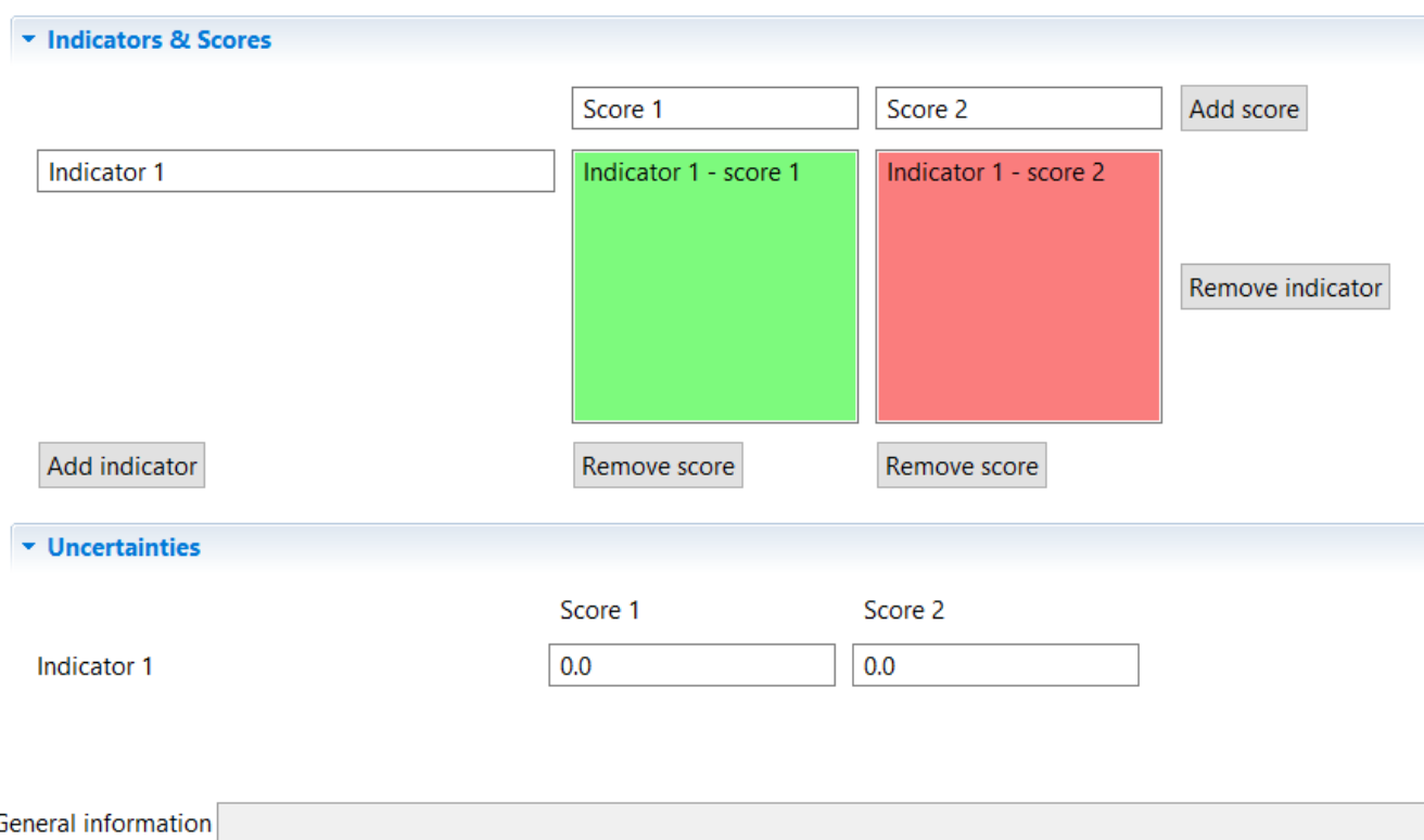
Figure 60: Create new data quality system, step 2
