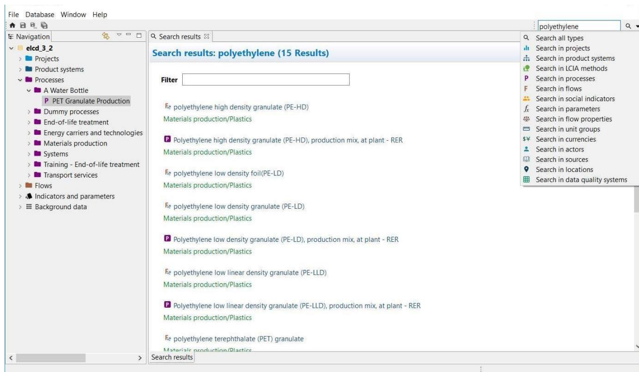
Figure 4.7: Search function
