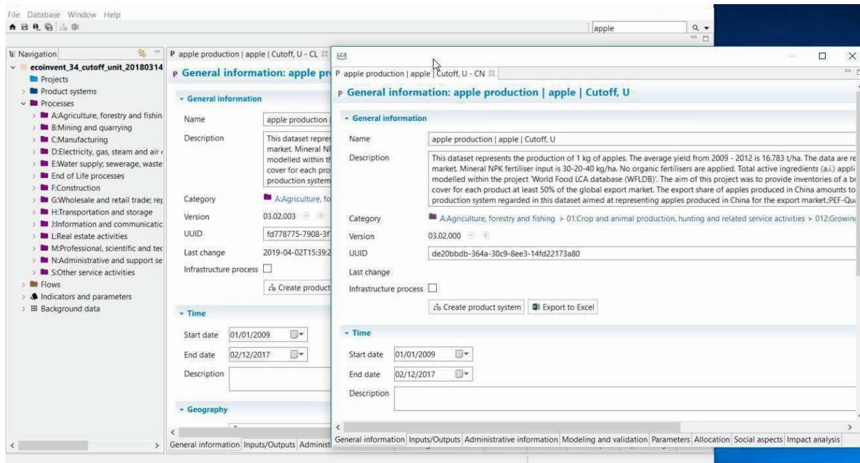
Figure 11.5: Detached windows
