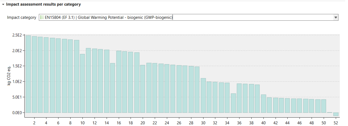
Figure 3-3 Dynamic GWP-biogenic results across lifetime of the building
