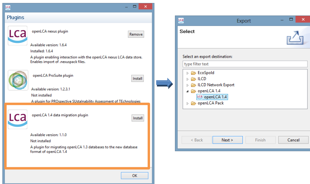
Figure 4. Migration of openLCA 1.3 databases (.olca) to openLCA 1.4 format (.zolca)
